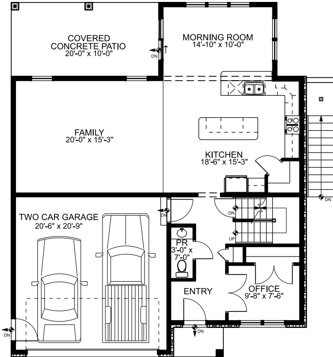
CEDAR CREEK ESTATES LOT NO. 252 1,148 SQ.FT. ROOM SIZES & SQUARE FOOTAGE FIGURES ARE APPROXIMATE REV. 09-MAR-21
